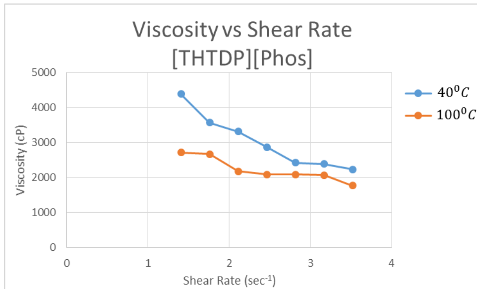
Figure 6: Viscosity of [THTDP][Phos] vs Shear Rate(sec -1 )
